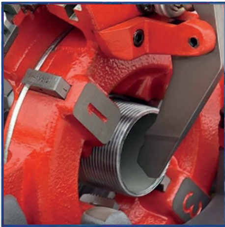
Pipe Threading
